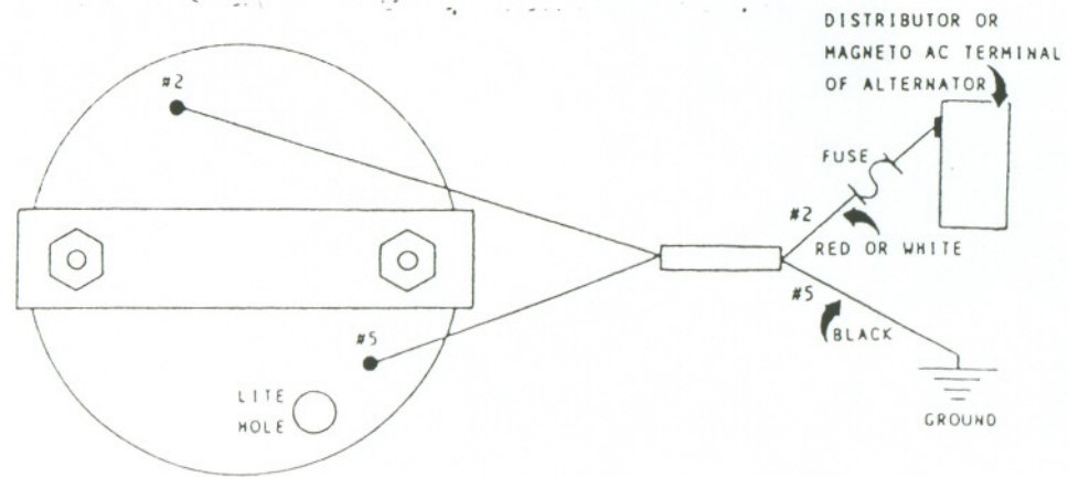
Show here is a common Tachometer Hook-up:
