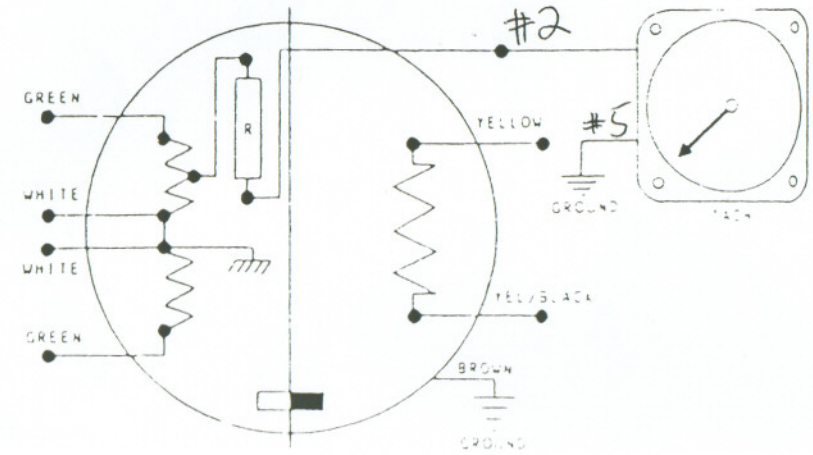
Wiring Diagram for Tachometer:
