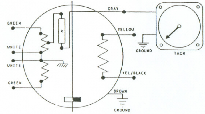
Wiring Diagram for Tachometer:
