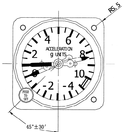
View A
